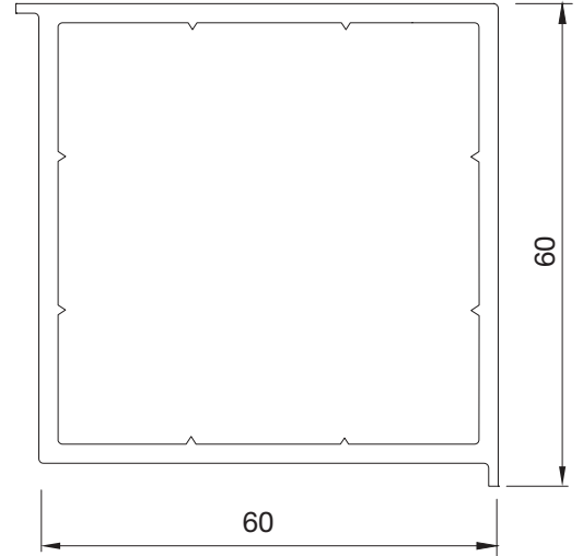
PEX3360BY.0003 60x60 KUTU 60x60 BOX
