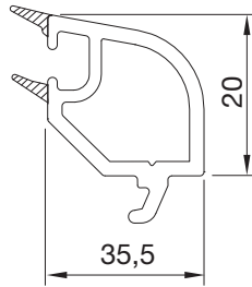
PVN1760BY.0001 20 mm CAM ÇİTASI 20 mm GLAZING BEAD
