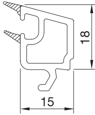
20 MM CAM ÇİTASI 20 MM GLAZING BEAD
