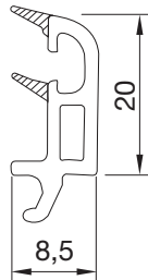
PS61760BY.0001 20 mm CAM ÇİTASI 20 mm GLAZING BEAD
