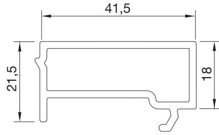
PSY4960BY.0001 INSERT INSERT
