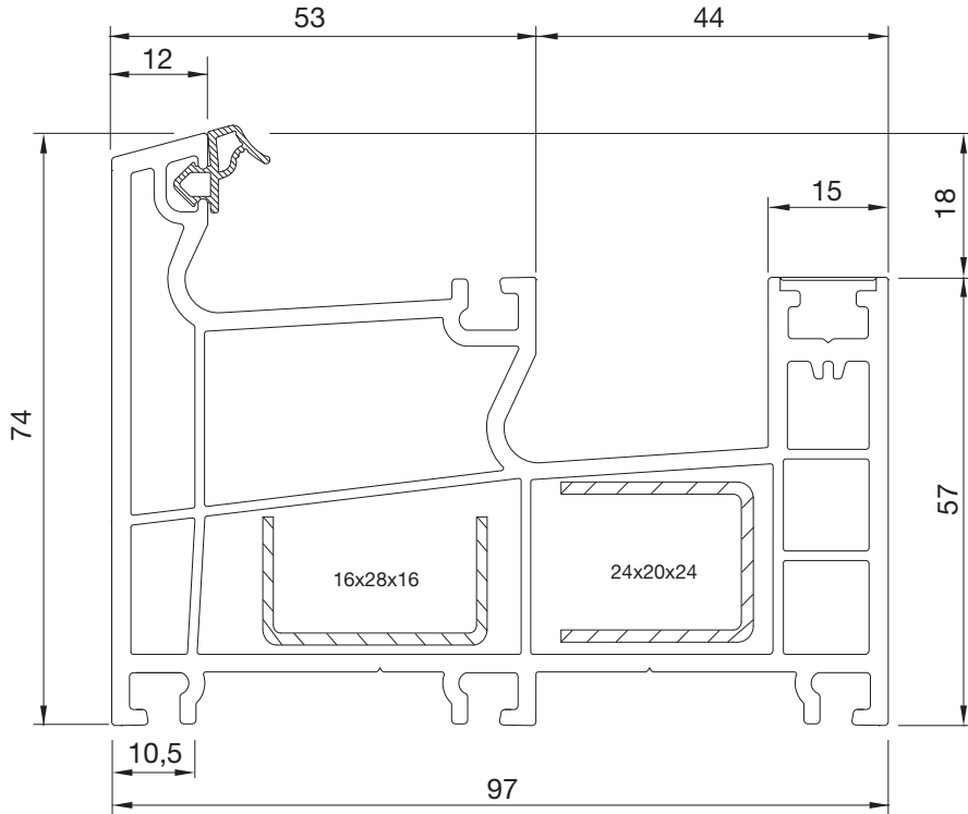
PSY5165BY.0001 DIŞ FIX KASA OUTSIDE FIX FRAME
