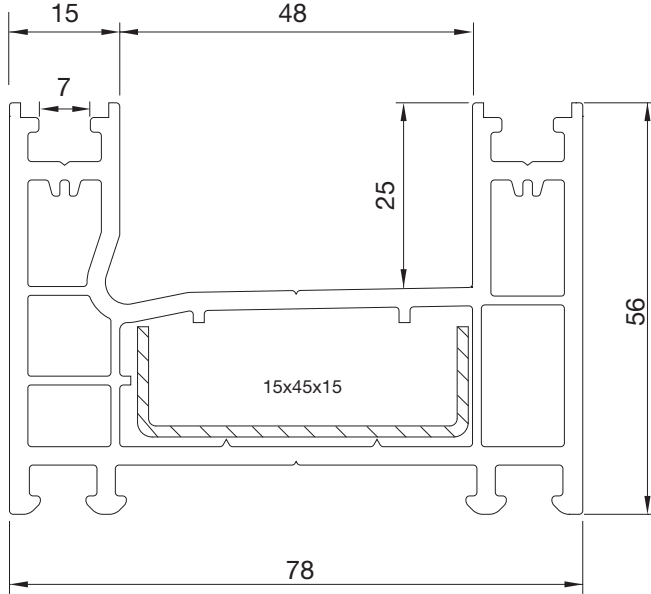
PSY0865BY.0001 PERVAZLI KASA CASING FRAME
