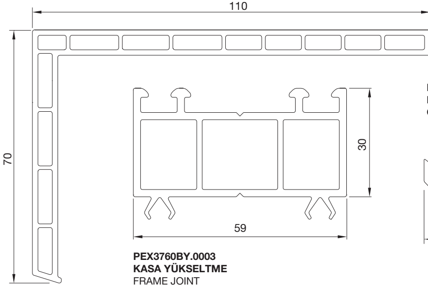
PTS3560BY PERVAZ PROFİLİ L TRIM PROFILE
