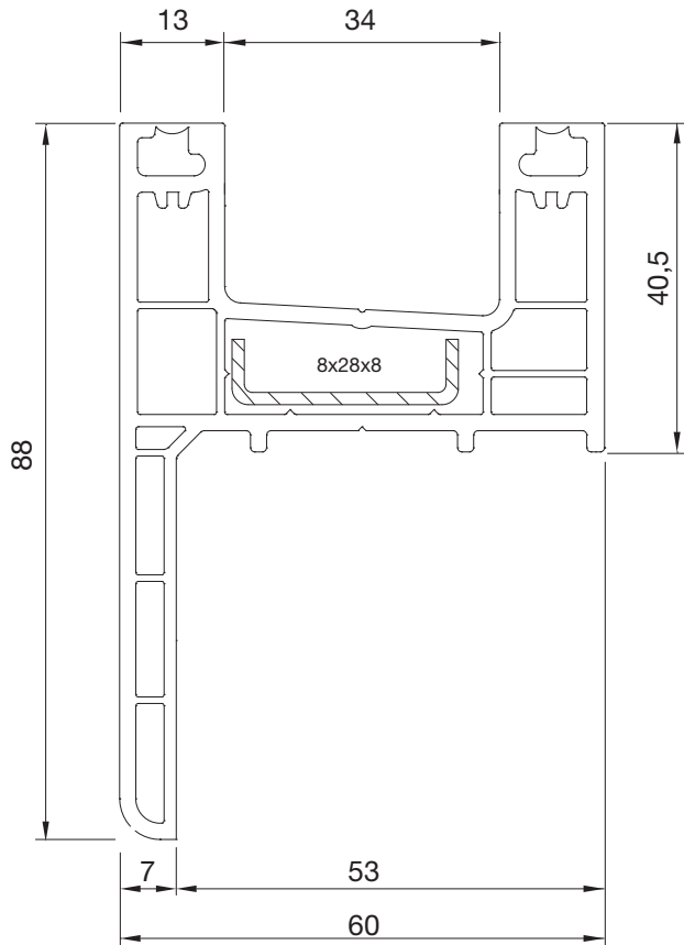
PS60865BY.0001 PERVAZLI KASA RENOVATION FRAME
