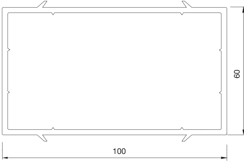
PEX3460BY.0003 100x60 KUTU 100x60 BOX
