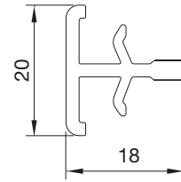
PTS2460BY.0003 İNCE BAĞ PROFİLİ COUPLING PROFILE
