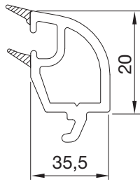
PVN1960BY.0001 24 mm CAM ÇİTASI 24 mm GLAZING BEAD
