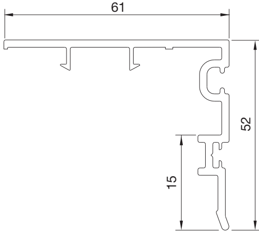
PTS3560BY PERVAZ PROFİLİ L TRIM PROFILE
