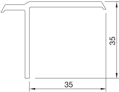
PTS3160BY ASİMETRİK T T COVERING
