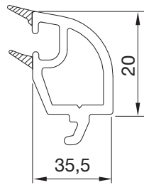
PVN1960BY.0001 24 mm CAM ÇİTASI 24 mm GLAZING BEAD
