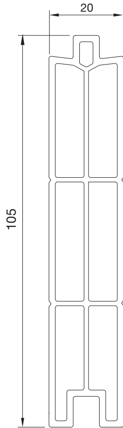
PTS2260BY.0003 LAMBRI 20 mm PANEL 20 mm
