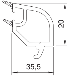
PVN1760BY.0001 TEK CAM ÇİTASI SINGLE GLAZING BEAD
