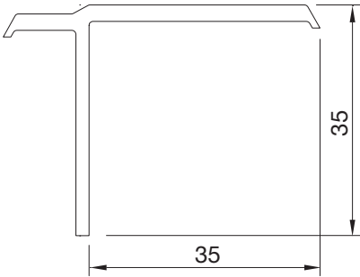
PTS3160BY ASİMETRİK T T COVERING
