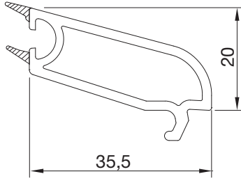
PVN1460BY.0001 TEK CAM ÇİTASI SINGLE GLAZING BEAD
