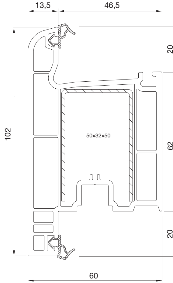
PVN0560BY.0003 DIŞA AÇILIM KAPI KANAT OUTSIDE OPENING DOOR SASH
