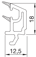
PEX1960BY.0001 24 MM CAM ÇİTASI 24 MM GLAZING BEAD
