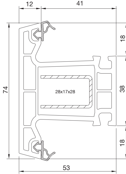
PFS0360BY.0001 ORTA KAYIT MULLION
