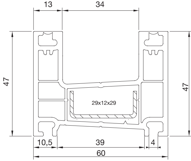
PS60165BY.0001 KASA FRAME
